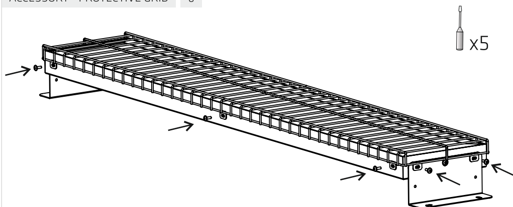
ACCESSORY - PROTECTIVE GRID 6
