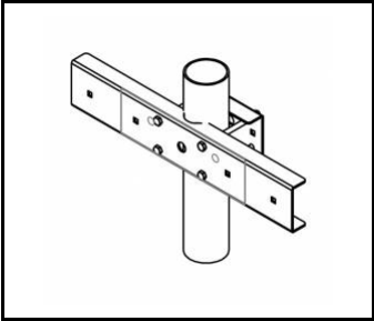
QUEST LED EVO S/M/L pole holder 1x (840401)
