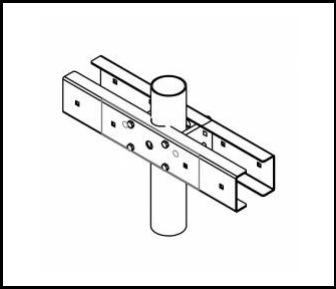
QUEST LED EVO S/M/L pole holder 2x (840418)
