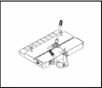
QUEST LED EVO S/M/L RCR Bausatz 1x (840388)
