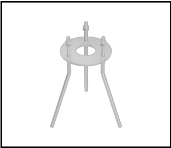
BOLLARD SKVER – Betonanker (498787)
